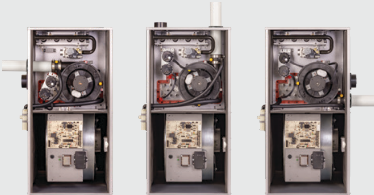
Upflow configurations
